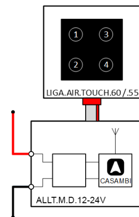
Touch panel with module
