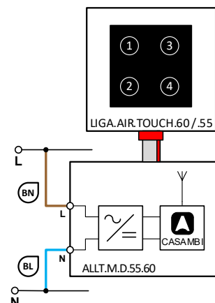
Touch panel with module
